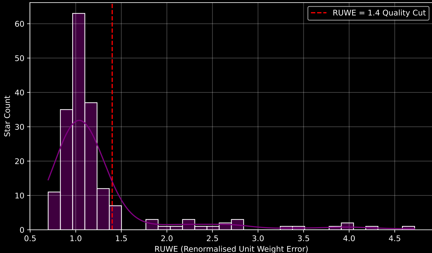
GALAH DR4 Field [7139] RUWE Distribution (n= 187)
