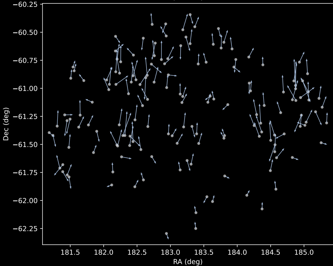
GALAH DR4 Cluster 1 Proper Motion Vectors (n=155)
