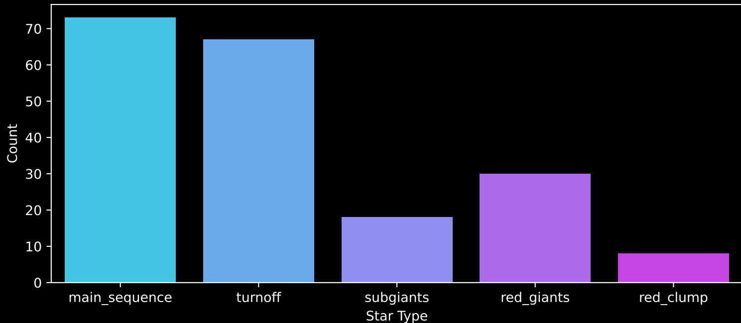
GALAH DR4 Field: [7139] Count plot of Star Type
