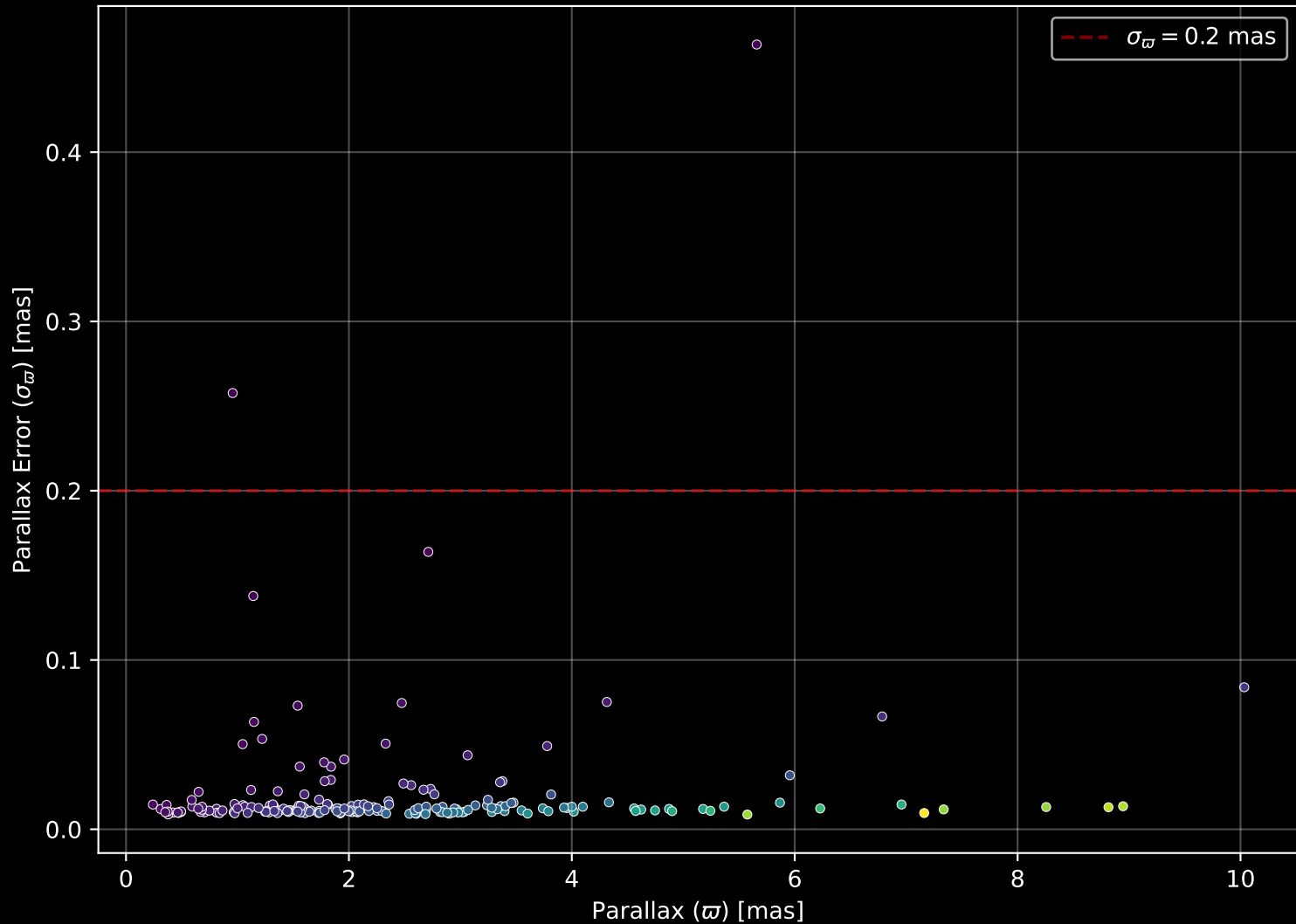
GALAH DR4 Field: [7139] Parallax Quality (n= 196)
