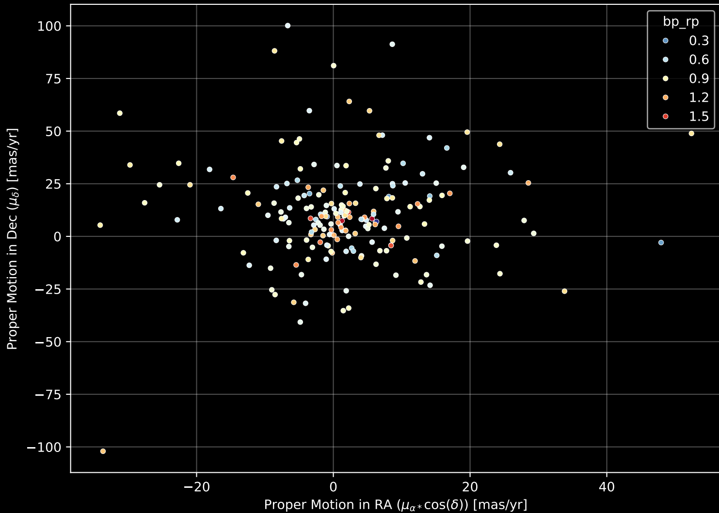
GALAH DR4 Field: [7139] Proper Motion Diagram (n= 196)
