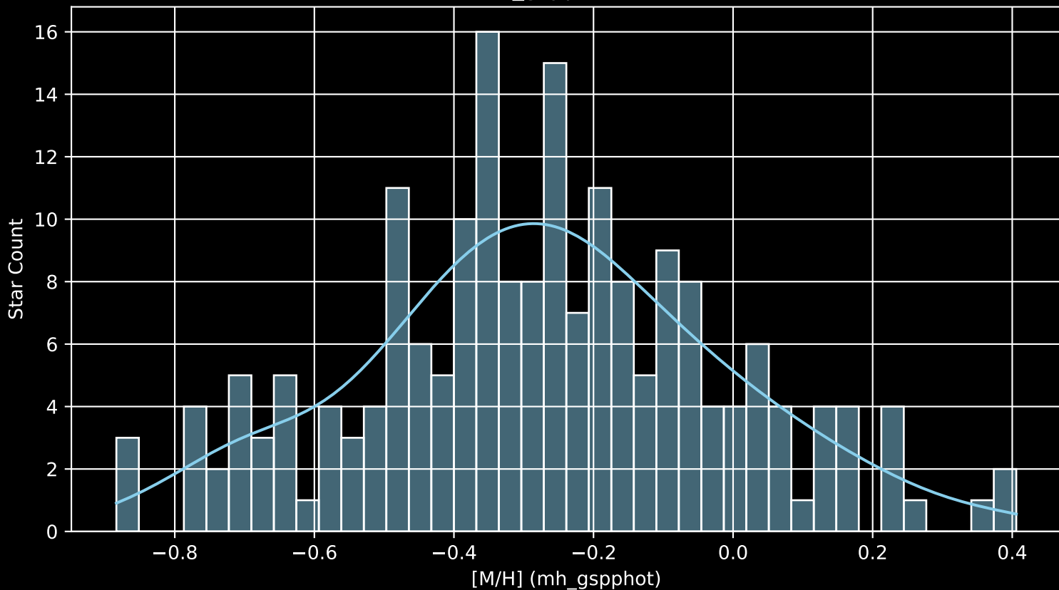
GALAH DR4 Field: [7139] [M/H] (mh_gspphot) (n= 196)
